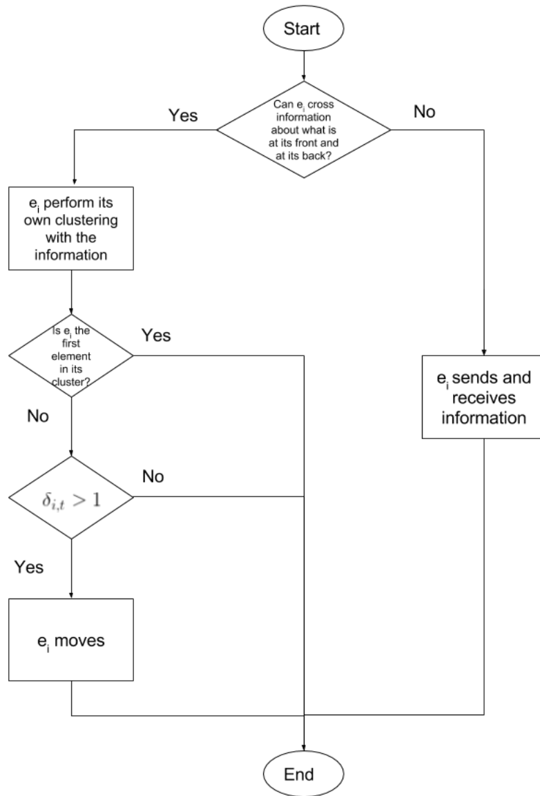
Figure 12: Model 4 flowchart
