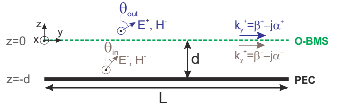
Fig. 1. Transversal section of the proposed LWA configuration, which consists of a parallel-plate waveguide with the top plate being a bianisotropic metasurface (O-BMS).
