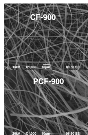
Figure 1. SEM images of CF-900 and PCF-900
