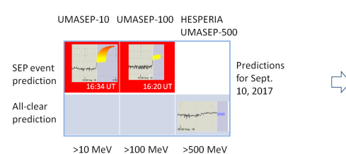
Figure 4. Summary of the >10, >100 and >500 MeV SEP forecast outputs of the UMASEP-based tools for the event that took place on Sept. 10 2017.
