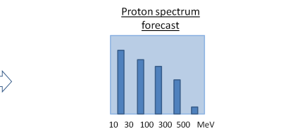
Figure 5. From the real-time UMASEP-based predictions of the occurrence and intensity of the first hours of >10 MeV, >100 MeV and >500 MeV SEP events presented in Figure 4, a real-time proton spectrum forecast might be constructed; this forecast output is our next goal.
