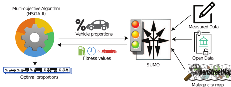
Fig. 1. System architecture.
