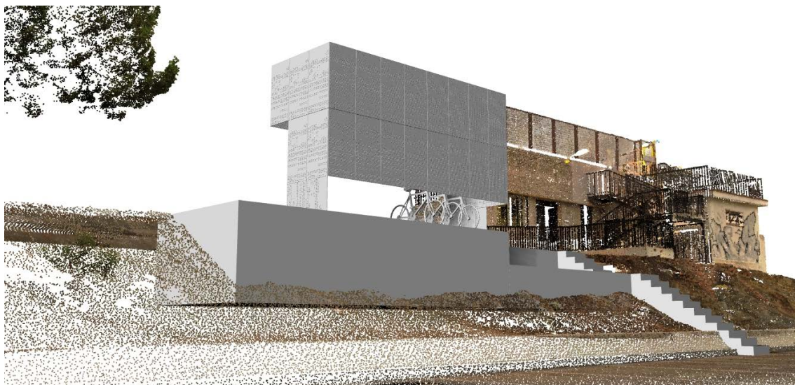
Figure 3. 3d rendering of the prototype implemented on a 3D laser scan of the site
