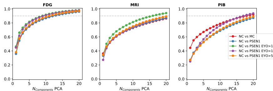
Figure 6: Cumulative variance of PCA relative to N_{\text{Comp}} .
