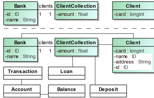
Fig. 2. Example of domain model: Bank class diagram
