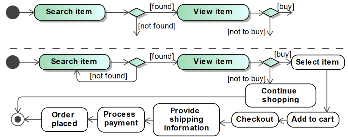
Fig. 5. Example of activity diagram: Online Shopping
