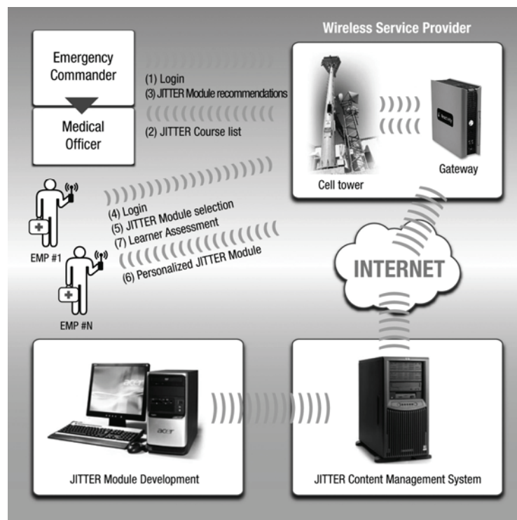
Figure 1. System architecture: organization of the different agents in distributing JITTER eTraining modules.
